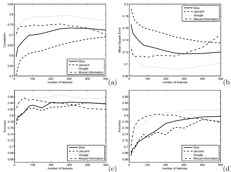
Fig. 1. Performance of affective lexicon creation as a function of the number of features (words) for the four similarity metrics. Results are shown (manually annotated scores stand as ground truth) for: (a) correlation between the automatically computed and manually annotated scores (ANEW corpus), (b) mean square error (ANEW), (c) binary (positive vs negative) classification accuracy (ANEW), (d) binary classification accuracy (General Inquirer).
