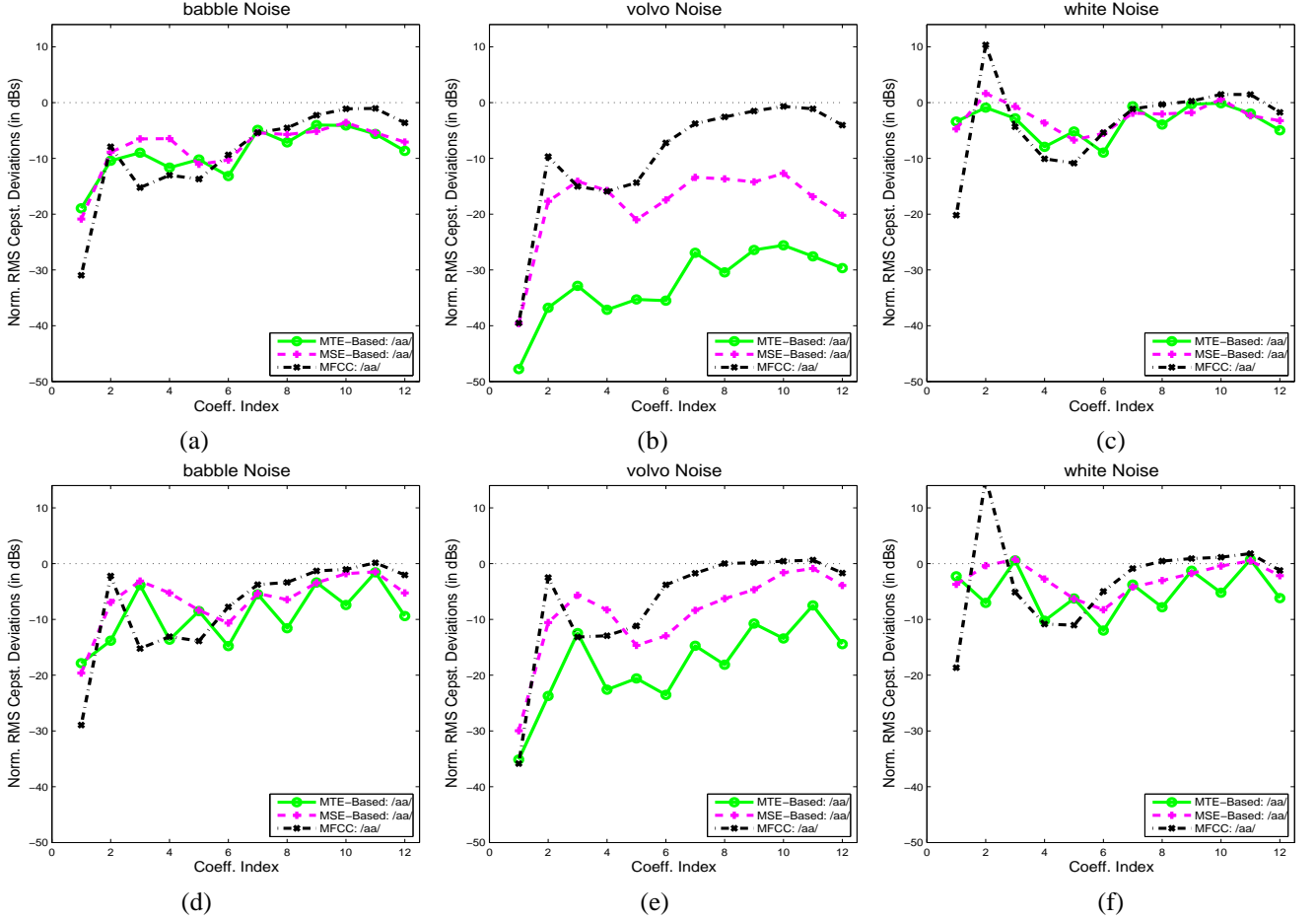
Fig. 4. Normalized RMS cepstral deviations (in dBs) computed over 1000 instances of the phoneme /aa/ extracted from the TIMIT database. Results shown as a function of coefficient index for babble (in (a),(d)), car (in (b),(e)) and white (in (c),(f)) noise at an average SNR = 5 dB. The filterbank consists of (a)-(c) 25 and (d)-(f) 100 mel-spaced, Gammatone filters with fixed overlap of 50%. Smaller values indicate enhanced robustness in noise.
