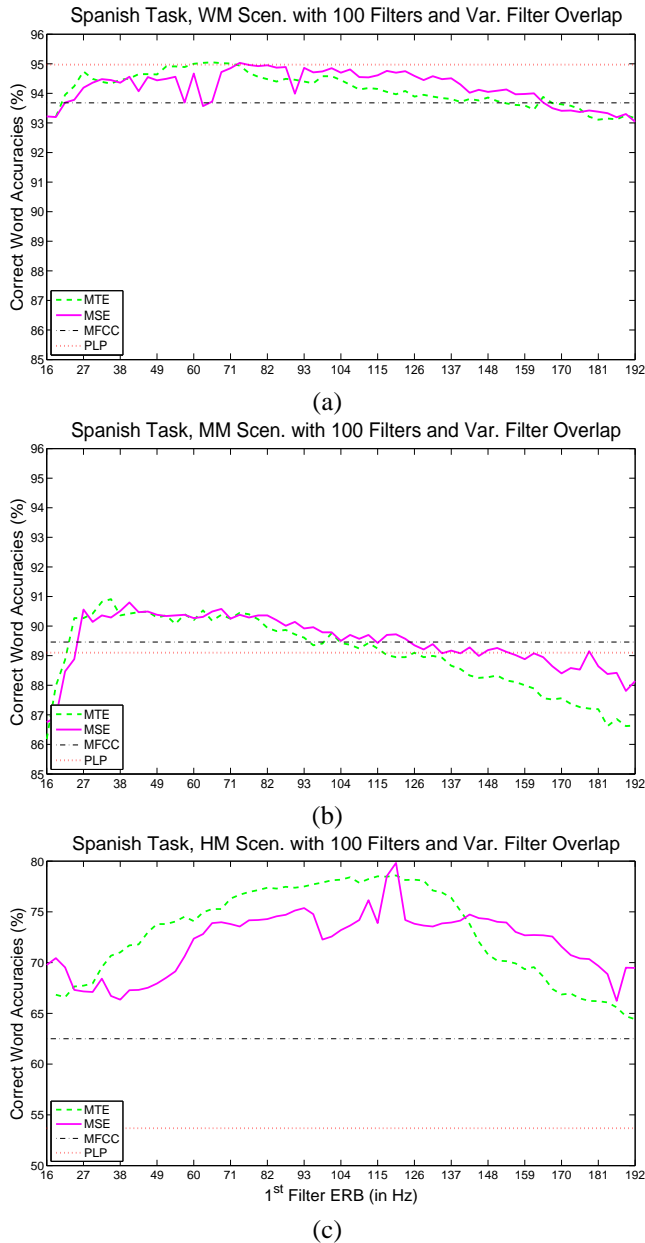
Fig. 5. Word accuracy for the cepstral MTE and MSE-based features (using CMS) for 100 Gammatone filters, in the Aurora-3 Spanish database. The horizontal axis displays the ERB Values of the 1 st filter. These values are equalized (sequentially) to the 1 st filter ERB values of the 25- and 50-filter filterbanks (when the filter overlap percent ranges in 30 – 85%). Results for three training/testing mismatched scenarios are shown: (a) High Mismatch (HM), (b) Medium Mismatch (MM), (c) Well Matched (WM). The baseline MFCC and PLP results are shown as dashed lines.
