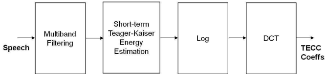
Fig. 1. Block Diagram of the TECC Feature Extraction Process.
