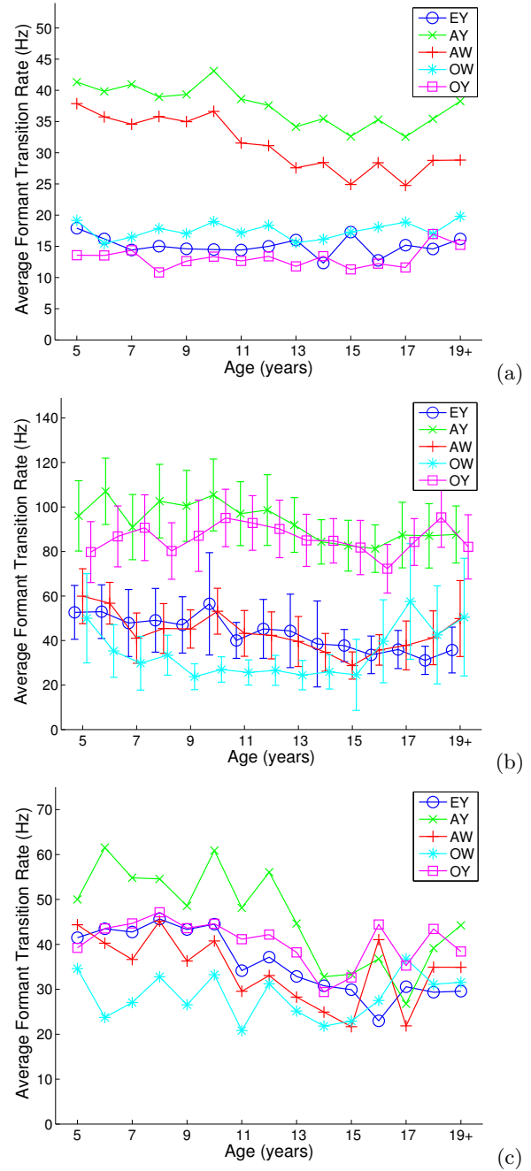
FIG. 6. Average formant transition rates for F1-F3 for each diphthong and age group (averaged over male and female subjects): (a) F1 average rate, (b) F2 average rate and standard deviation, (c) F3 average rate.
