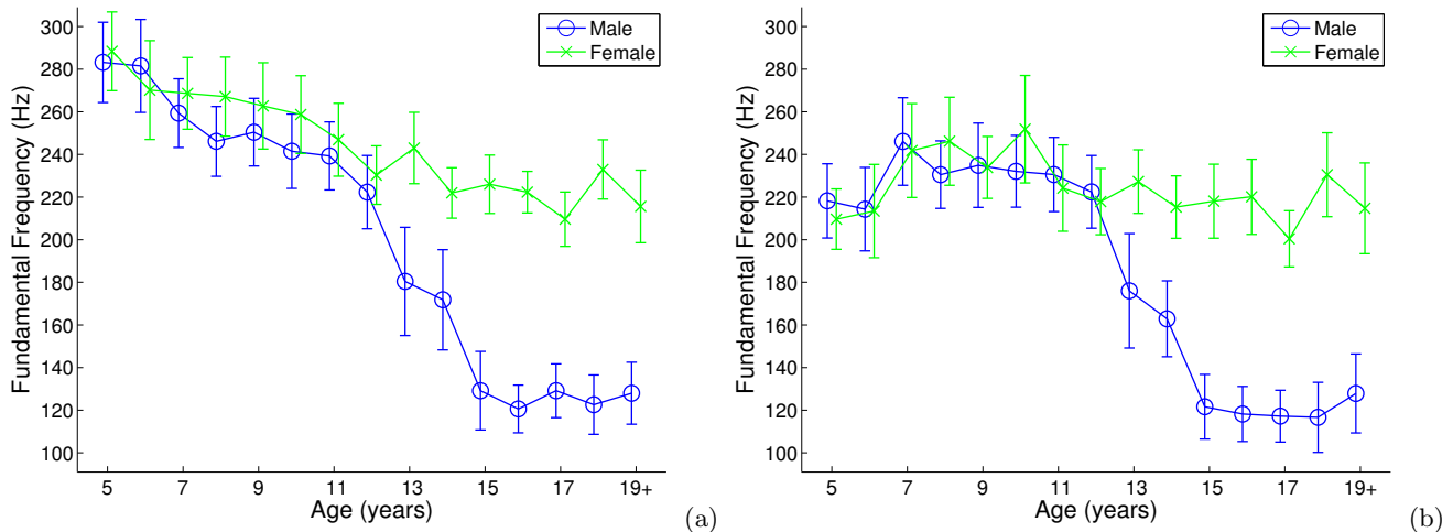
FIG. 3. Average fundamental frequency for male and female subjects measured at: (a) diphthong onset, (b) diphthong offset.
