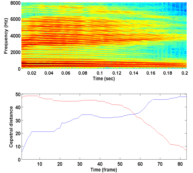
FIG. 1. Example of front-back cepstral distances to estimate a spectral transition mid-point (bottom) together with the corresponding narrow-band spectrogram (top). Token is /AY/ produced by a child of age 5 years.
