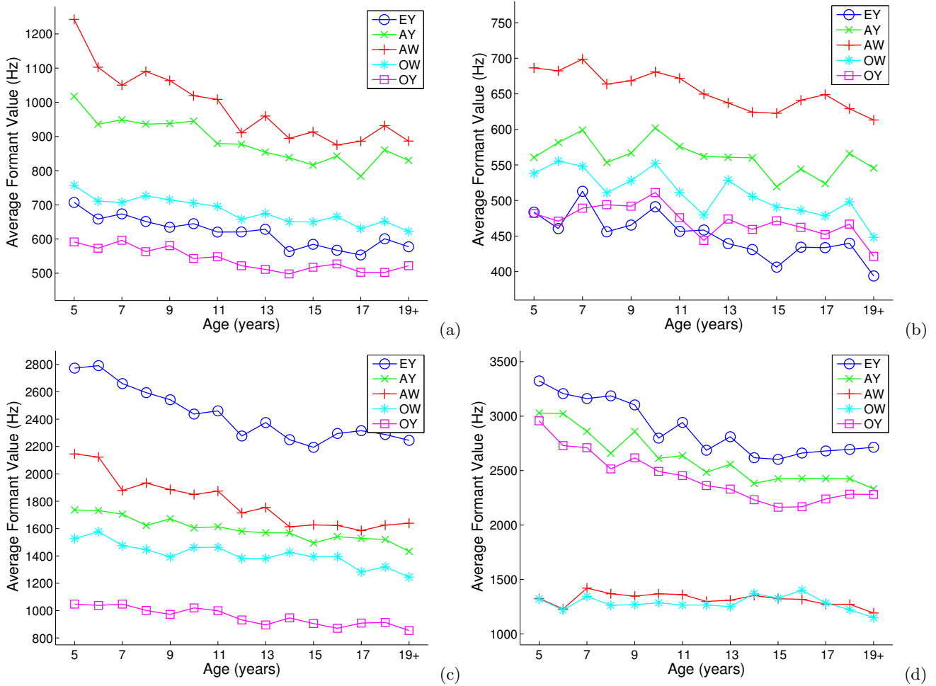
FIG. 5. Average formant values for female subjects as a function of age group and diphthong: (a) F1 at dipthong onset, (b) F1 at dipthong offset, (c) F2 at dipthong onset, and (d) F2 at dipthong offset.
