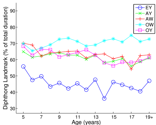
FIG. 9. Diphthong landmark (transitional mid-points) for each age group and diphthong.
