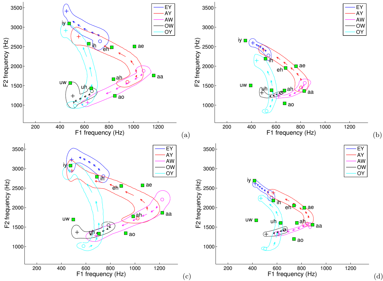
FIG. 7. Five diphthong trajectories are represented by five colored “strips” in which arrows represent trajectory midline segments between onset (‘o’) and offset (‘x’) positions, and strip width corresponds to formant variability at selected locations along the midline. Plots are for: (a) male age 5, (b) male age 14, (c) female age 5, and (d) female age 14. Formant positions of 9 monophthongs (squares with two-character ARPABET vowel symbols) of each age group are also shown in background for comparison to onsets and offsets of diphthongs. It is clear that the positional relationship between diphthong onsets and offsets and nearby monophthongs are different between the two age groups.
