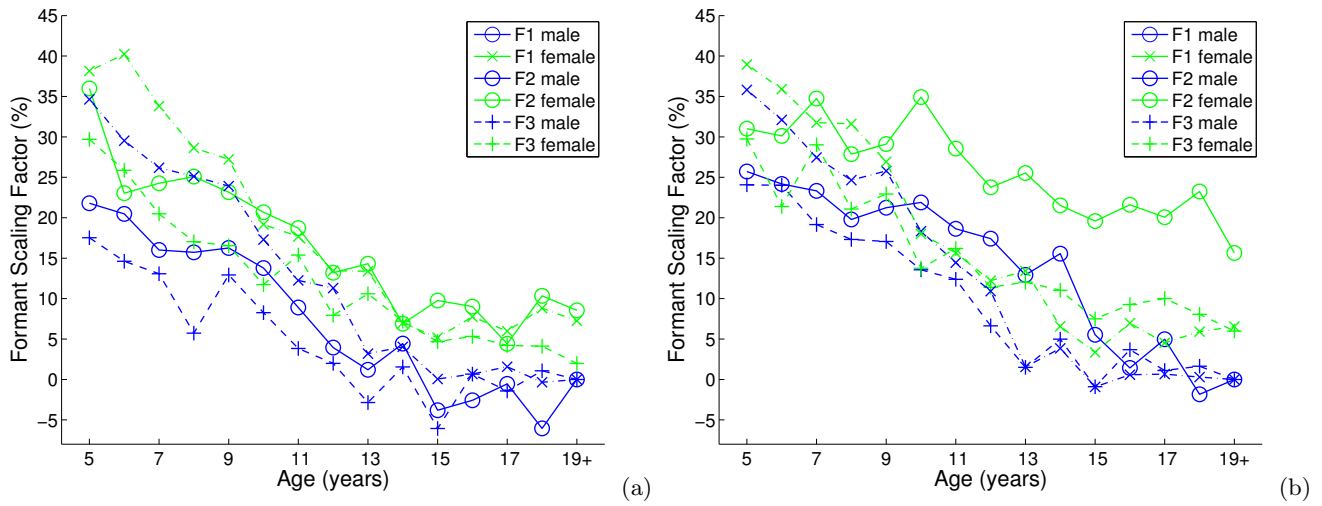
FIG. 4. Average formant scaling factors for F1-F3 male and female subjects measured at: (a) dipthong onset, (b) dipthong offset. Scaling is computed relative to adult male formant frequency values.
