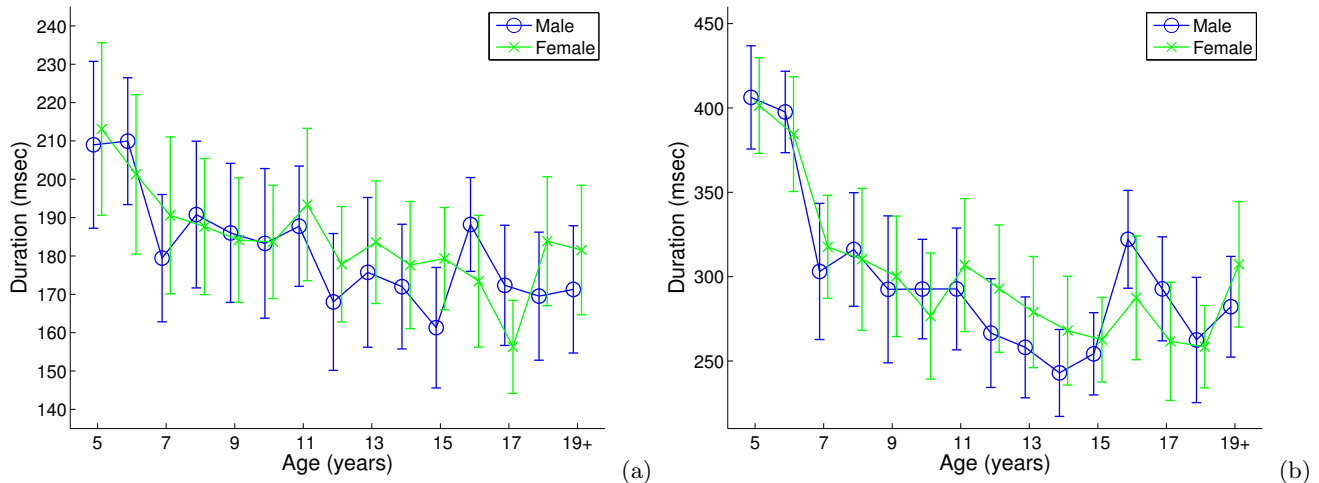
FIG. 2. (a) Averaged durations for diphthongs /EY/, /AY/, /AW/, /OW/ for male and female subjects in each age group. (b) Averaged duration for diphthong /OY/ per gender and age group. Note that the y-axis scale is different due to the difference in dynamic range of values in the two plots.
