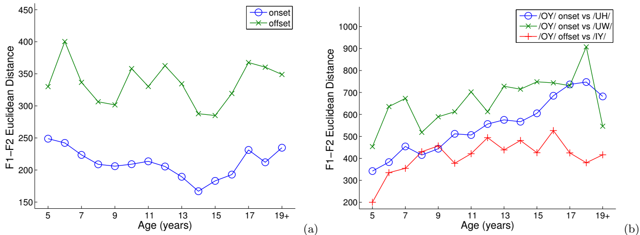
FIG. 8. Average F1-F2 Euclidean distances between onsets and offsets of diphthongs and corresponding monophthongs as a function of age: (a) averages over diphthongs /EY/, /AY/, /AW/, /OW/ and (b) /OY/.
